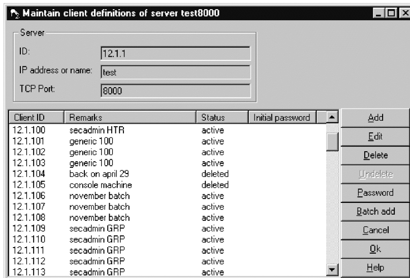
Figure 76. Maintain Client window
