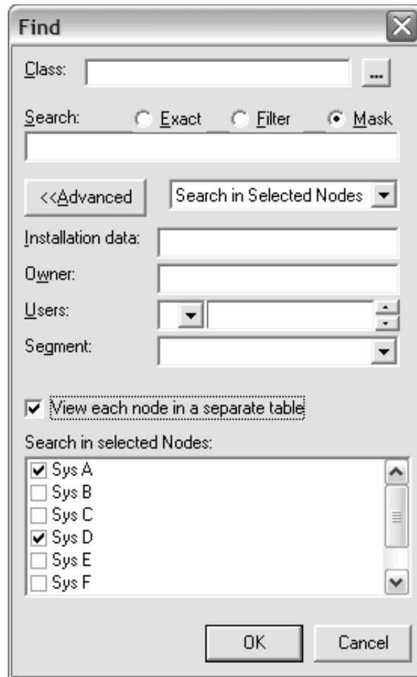
Figure 11. Find dialog
