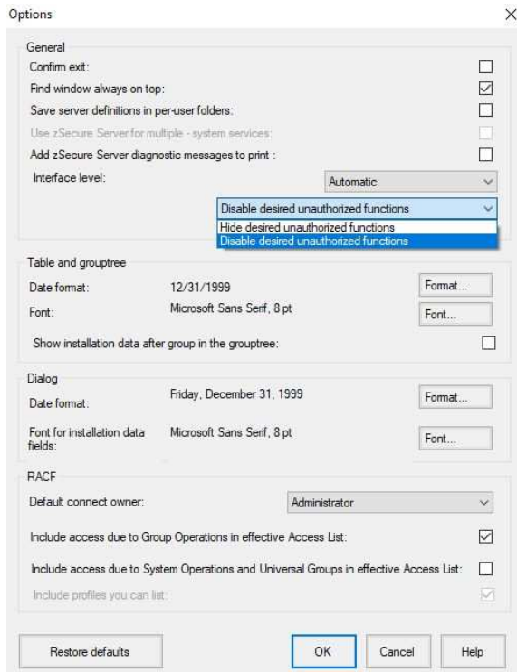
Figure 7. Options dialog
